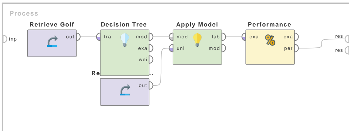
Figure 6.19: Tutorial process 'Applying the Performance (Ranking) operator on the Golf data set'.
