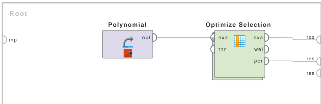
Figure 4.109: Tutorial process 'Feature reduction of the Polynomial data set'.
