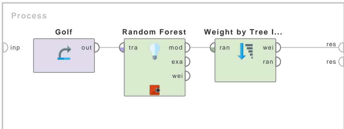
Figure 4.99: Tutorial process 'Calculating the attribute weights of the Golf data set using Random Forest model'.
