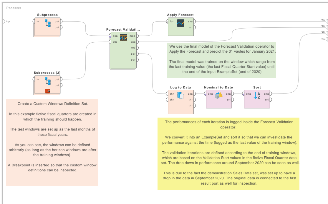
Figure 4.167: Tutorial process 'Use custom windowing to define your own training and test windows'.
