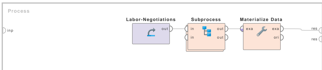
Figure 7.86: Tutorial process 'Creating fresh copy of an ExampleSet'.
