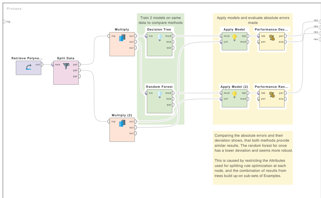
Figure 4.24: Tutorial process ‘Comparison between decision tree and random forest’.
