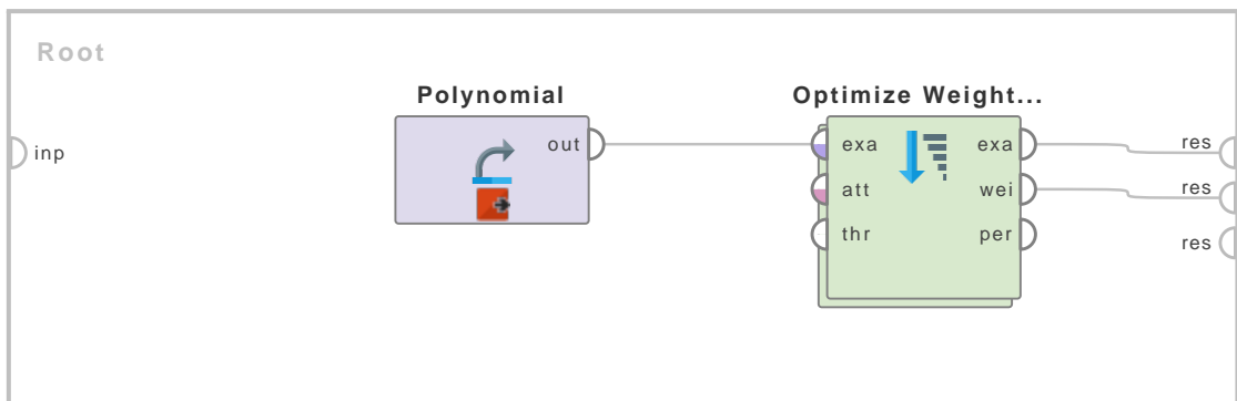
Figure 4.115: Tutorial process 'Calculating the weights of the attributes of the Polynomial data set'.
