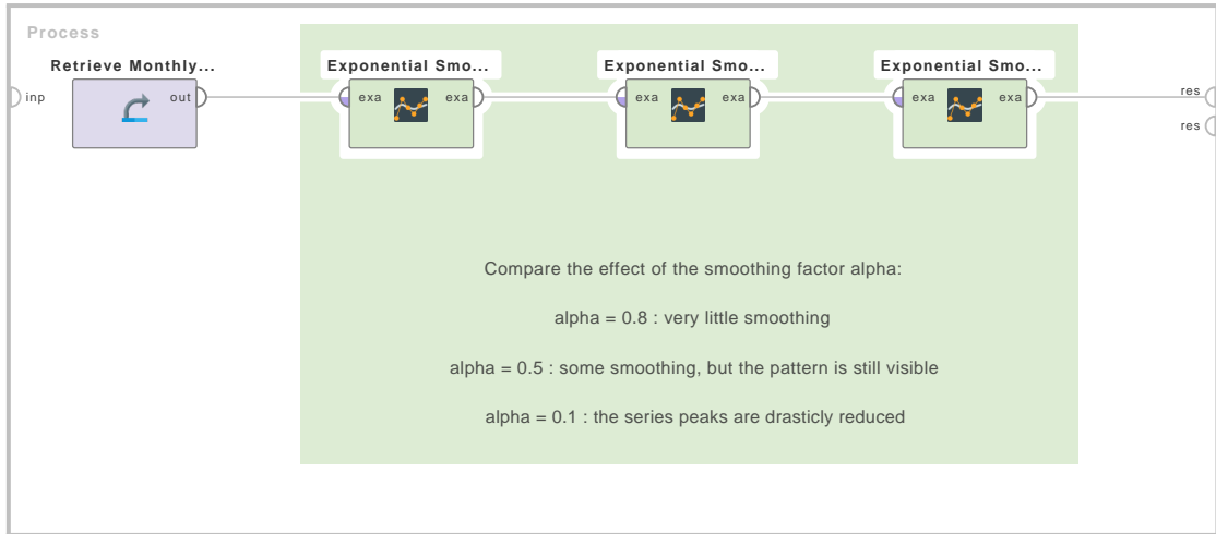
Figure 4.125: Tutorial process 'Exponential Smoothing'.
