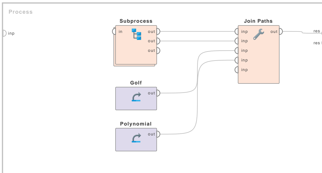
Figure 7.85: Tutorial process 'Returning the first non-null object'.
