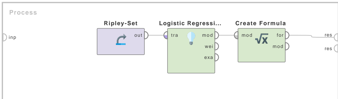
Figure 4.3: Tutorial process 'Formula of the Logistic Regression model'.
