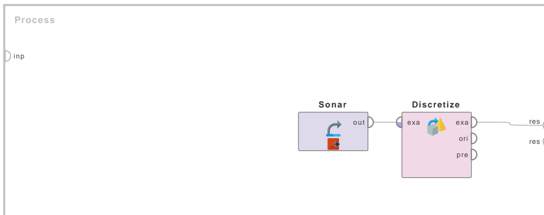
Figure 3.4: Tutorial process 'Discretizing the 'Sonar' data set by entropy'.
